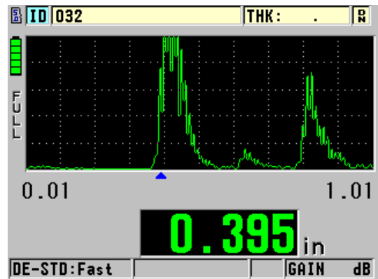
Indoor display setting, optional A-scan mode
