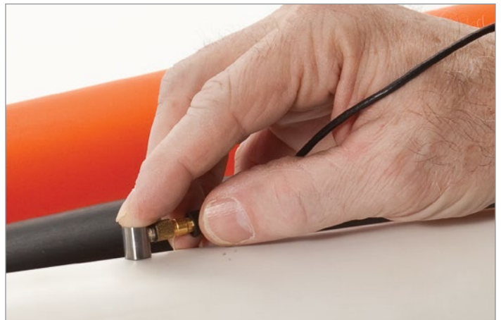
Measure the thickness of many materials including plastic, metal, rubber, glass, ceramic, and composites.
